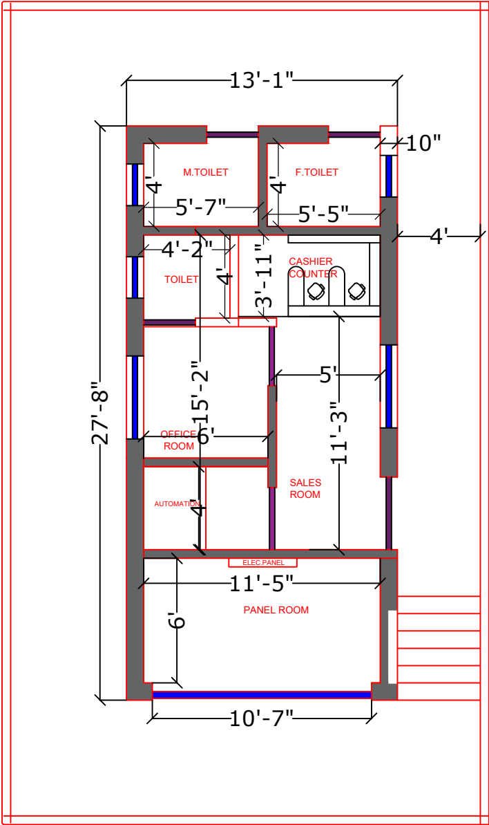
GROUND FLOOR PLAN North
